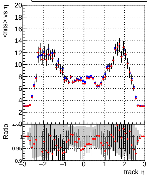
mean hits vs \eta Legend: DQM_CKF_TTbase (blue line with error bars), DQM_CKF_TT_retrainOldFiles125_v2_prelimWP3_epoch4 (red line with error bars)
