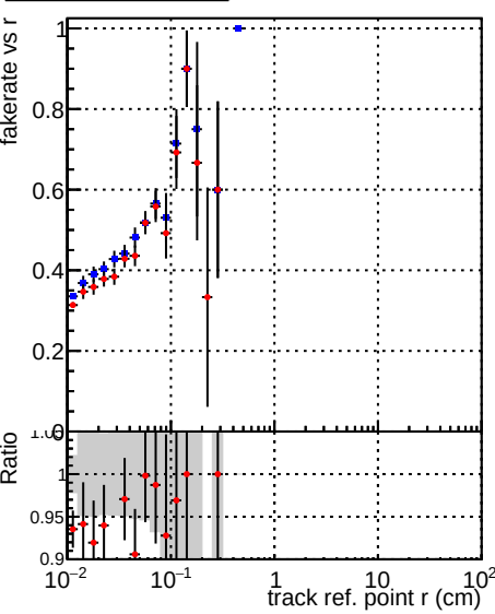
Fake rate vs v DQM_CKF_TTbase DQM_CKF_TT_retrainOldFiles125_v2_prelimWP3_epoch4
