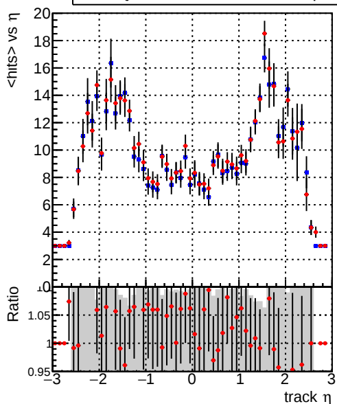
mean hits vs \eta Legend: DQM_CKF_TTbase (blue line with dots), DQM_CKF_TT_retrainOldFiles125_v2_prelimWP3_epoch4 (red line with dots)
