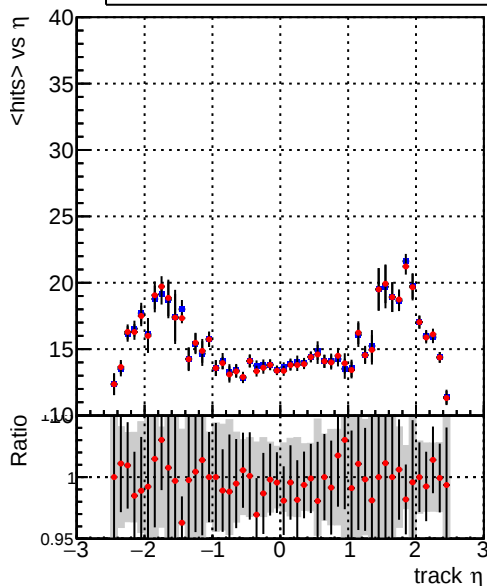
mean hit \eta Legend: DQM_CKF_TTbase (blue line), DQM_CKF_TT_retrainOldFiles125_v2_prelimWP3_epoch4 (red line)
