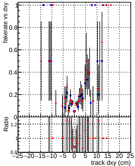
—●— DQM_CKF_TTbase —●— DQM_CKF_TT_retrainOldFiles125_v2_prelimWP3_epoch4
