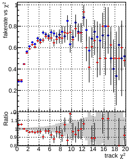
Fake rate vs. \chi^2 for DQM CKF TTbase and DQM CKF TT_retrainOldFiles125_v2_prelimWP3_epoch4
