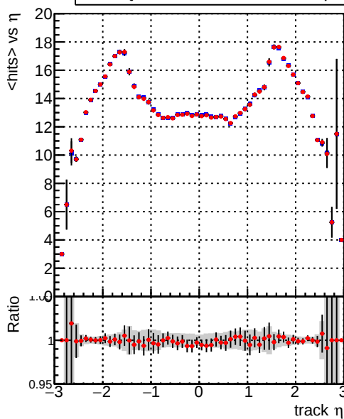
— DQM_CKF_TTbase — DQM_CKF_TT_retrainOldFiles125_v2_prelimWP3_epoch4 mean hits vs \eta
