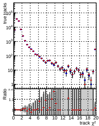
N of reco track vs. \chi^2 DQM_CKF_TTbase DQM_CKF_TT_retrainOldFiles25_v2_prelimWP3_epoch4
