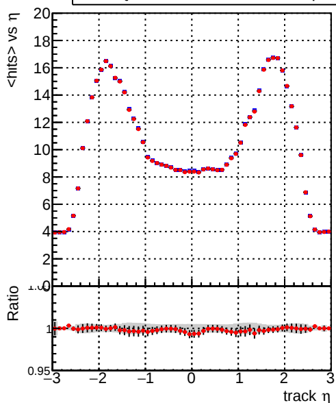
— DQM_CKF_TTbase — DQM_CKF_TT_retrainOldFiles125_v2_prelimWP3_epoch4
