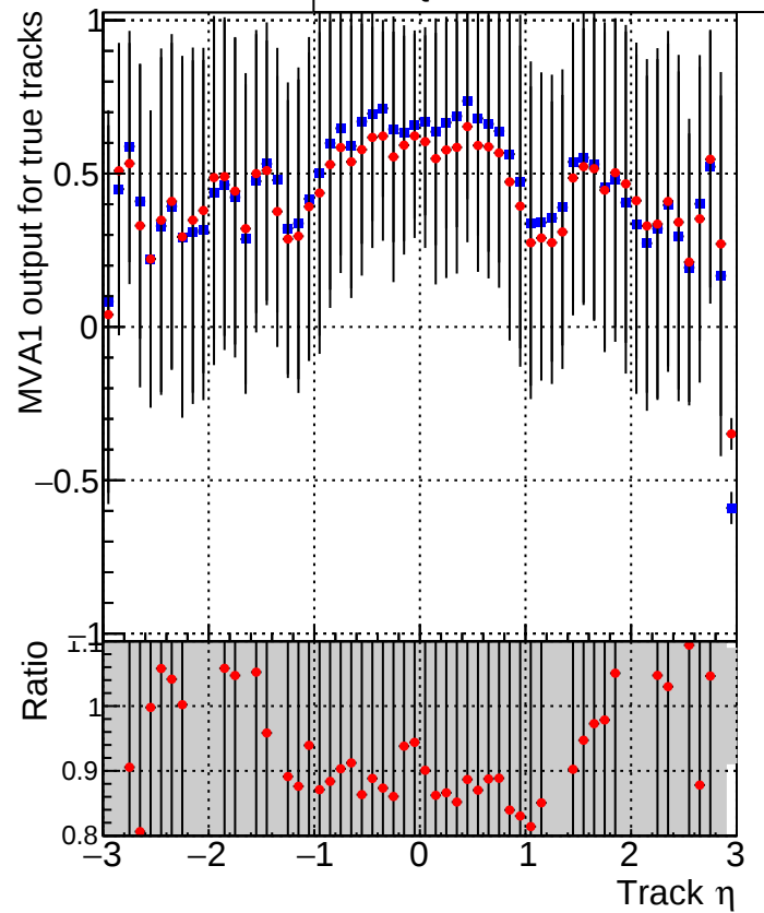
MVA1 of associated tracks (recoToSim) vs. track \eta Legend: ■ DQM_CKF_TTbase ● DQM_CKF_TT_retrainOldFiles125_v2_prelimWP3_epoch4
