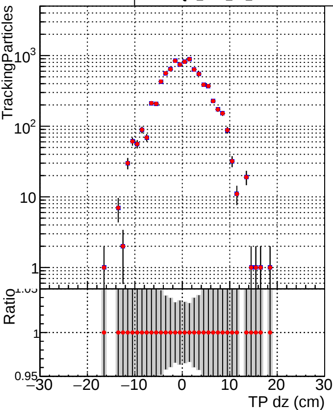
■ DQM_CKF_TTbase ● DQM_CKF_TT_retrainOldFiles125_v2_prelimWP3_epoch4
