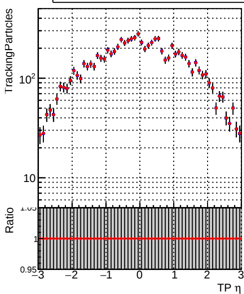
N of simulated tracks vs \eta Legend: DQM_CKF_TTbase (blue diamonds), DQM_CKF_TT_retrainOldFiles125_v2_prelimWP3_epoch4 (red diamonds)
