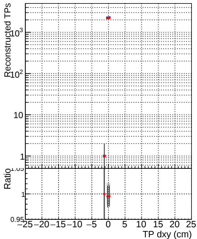
■ DQM_CKF_TTbase ● DQM_CKF_TT_retrainOldFiles125_v2_prelimWP3_epoch4
