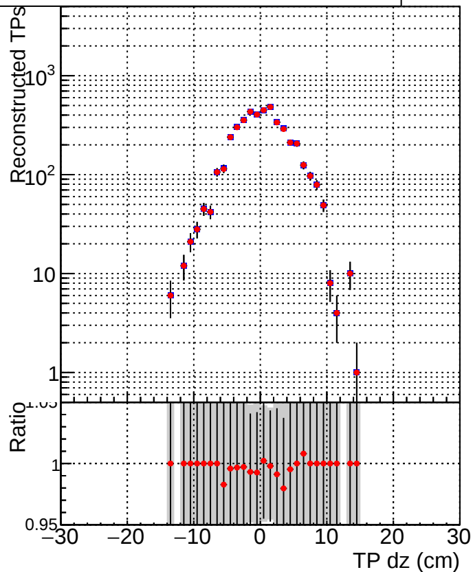
■ DQM_CKF_TTbase ● DQM_CKF_TT_retrainOldFiles125_v2_prelimWP3_epoch4
