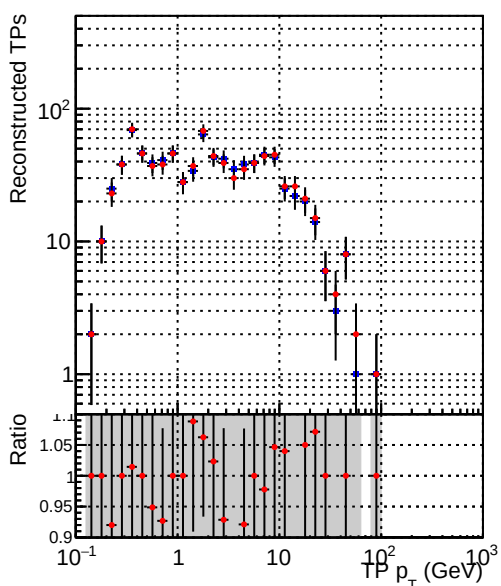
—●— DQM_CKF_TTbase —●— DQM_CKF_TT_retrainOldFiles125_v2_prelimWP3_epoch4
