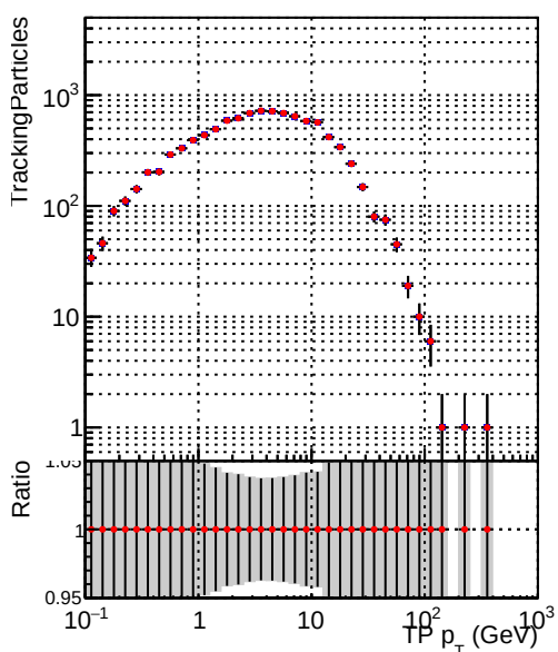
—●— DQM_CKF_TTbase —●— DQM_CKF_TT_retrainOldFiles125_v2_prelimWP3_epoch4
