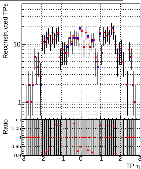
—●— DQM_CKF_TTbase —●— DQM_CKF_TT_retrainOldFiles125_v2_prelimWP3_epoch4
