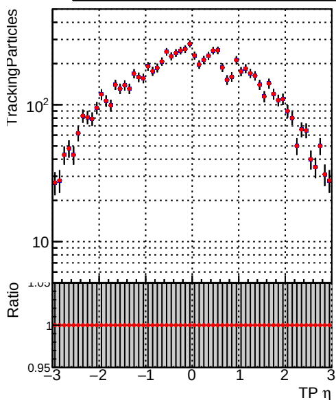
—●— DQM_CKF_TTbase —●— DQM_CKF_TT_retrainOldFiles125_v2_prelimWP3_epoch4
