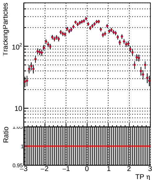
— DQM_CKF_TTbase — DQM_CKF_TT_retrainOldFiles125_v2_prelimWP3_epoch4
