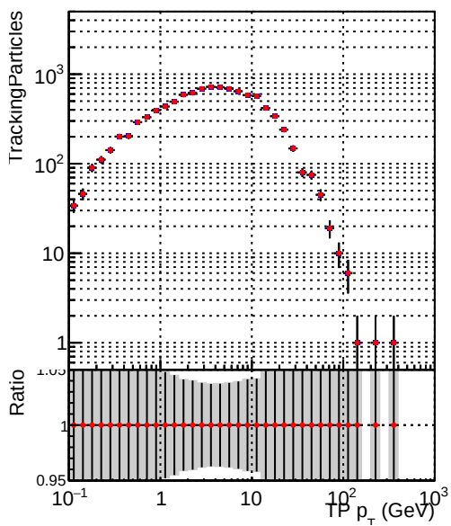
— DQM_CKF_TTbase — DQM_CKF_TT_retrainOldFiles125_v2_prelimWP3_epoch4
