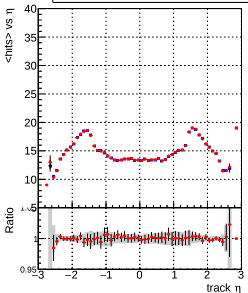
mean hits vs \eta — DQM_CKF_TTbase — DQM_CKF_TT_retrainOldFiles125_v2_prelimWP3_epoch4
