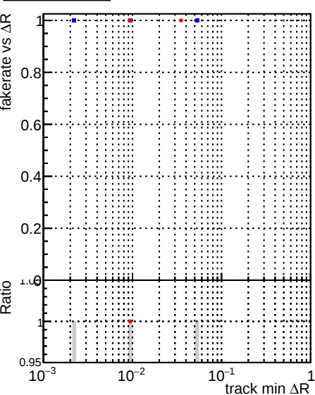
Fake rate vs ΔR(track, jet) Legend: DQM_CKF_TTbase (blue squares) DQM_CKF_TT_retrainOldFiles125_v2_prelimWP3_epoch4 (red circles)
