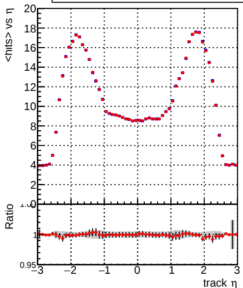
— DQM_CKF_TTbase — DQM_CKF_TT_retrainOldFiles125_v2_prelimWP3_epoch4 mean hits
