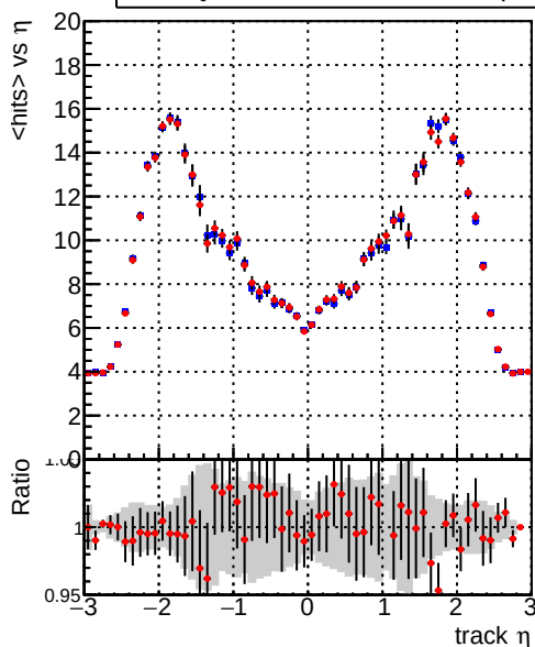
— DQM_CKF_TTbase — DQM_CKF_TT_retrainOldFiles125_v2_prelimWP3_epoch4
