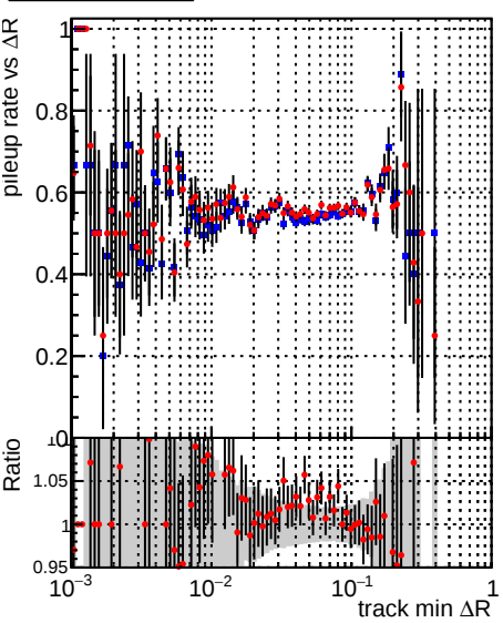
■ DQM_CKF_TTbase ● DQM_CKF_TT_retrainOldFiles125_v2_prelimWP3_epoch4
