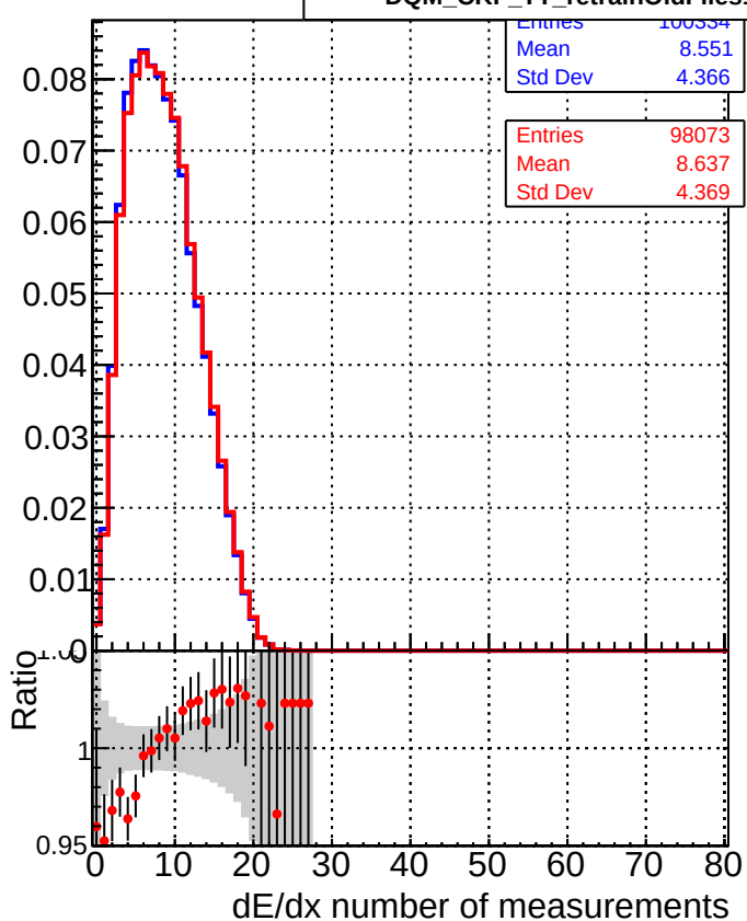
Legend: DQM_CKF_TTbase (blue line with squares) DQM_CKF_TT_retrainOldFiles125_v2_prelimWP3_epoch4 (red line with circles)
