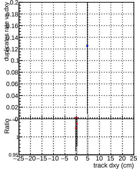
—●— DQM_CKF_TTbase —●— DQM_CKF_TT_retrainOldFiles125_v2_prelimWP3_epoch4
