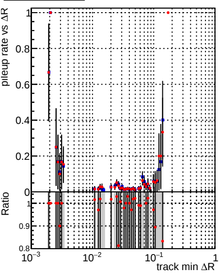
Legend: DQM_CKF_TTbase (blue squares), DQM_CKF_TT_retrainOldFiles125_v2_prelimWP3_epoch4 (red circles)
