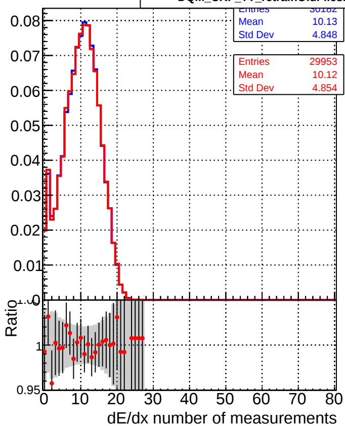
— DQM_CKF_TTbase — DQM_CKF_TT_retrainOldFiles125_v2_prelimWP3_epoch4
