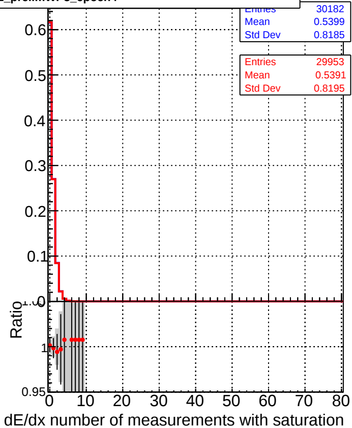
— DQM_CKF_TTbase — DQM_CKF_TT_retrainOldFiles125_v2_prelimWP3_epoch4
