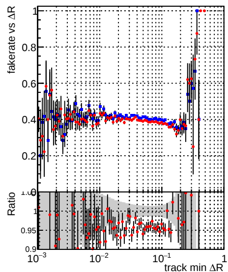
Legend: DQM_CKF_TTbase (blue), DQM_CKF_TT_retrainOldFiles125_v2_prelimWP3_epoch4 (red)
