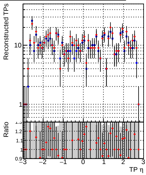
■ DQM_CKF_TTbase ● DQM_CKF_TT_retrainOldFiles125_v2_prelimWP3_epoch4
