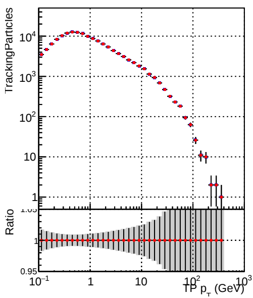
■ DQM_CKF_TTbase ● DQM_CKF_TT_retrainOldFiles125_v2_prelimWP3_epoch4
