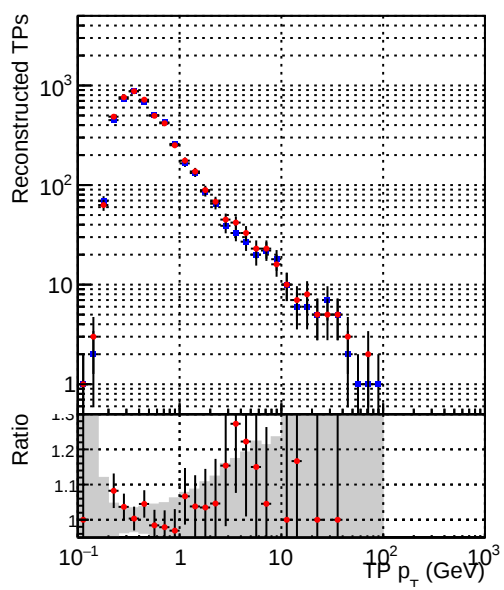
■ DQM_CKF_TTbase ● DQM_CKF_TT_retrainOldFiles125_v2_prelimWP3_epoch4
