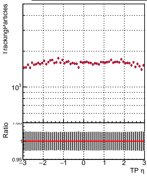
N of simulated tracks vs \eta Legend: — DQM_CKF_TTbase — DQM_CKF_TT_retrainOldFiles125_v2_prelimWP2_epoch4
