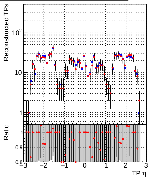
—•— DQM_CKF_TTbase —•— DQM_CKF_TT_retrainOldFiles125_v2_prelimWP2_epoch4
