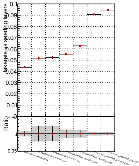
Fake rate vs. —•— DQM_CKF_TTbase —•— DQM_CKF_TT_retrainOldFiles125_v2_prelimWP2_epoch4
