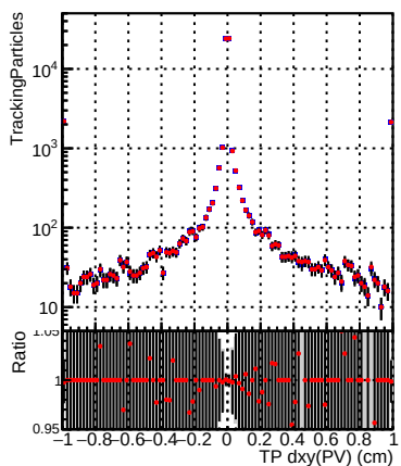
N of sim DQM_CKF_TT_retrainOldFiles125_v2_prelimWP2_epoch4
