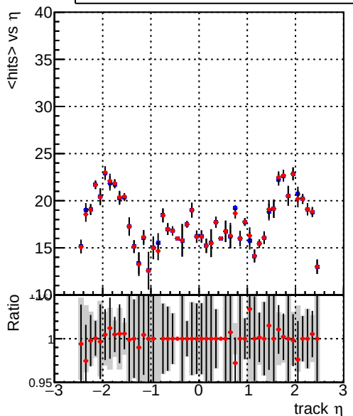
mean hits — DQM_CKF_TTbase — DQM_CKF_TT_retrainOldFiles125_v2_prelimWP2_epoch4
