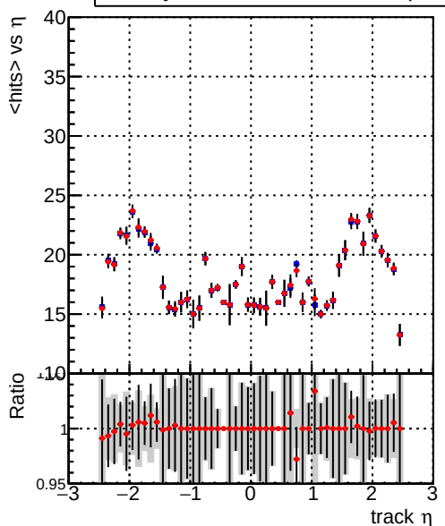
Legend: — DQM_CKF_TTbase, — DQM_CKF_TT_retrainOldFiles125_v2_prelimWP2_epoch4 mean hits vs \eta
