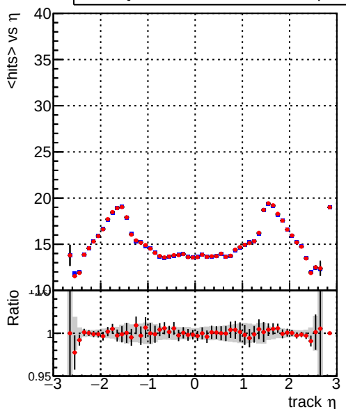
mean hits vs \eta Legend: DQM_CKF_TTbase (blue line), DQM_CKF_TT_retrainOldFiles125_v2_prelimWP2_epoch4 (red line)
