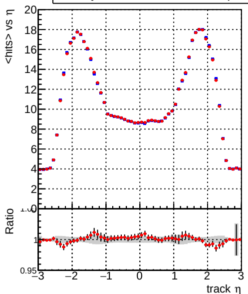
mean hits vs \eta — DQM_CKF_TTbase — DQM_CKF_TT_retrainOldFiles125_v2_prelimWP2_epoch4
