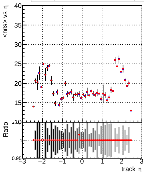
mean hits — DQM_CKF_TTbase — DQM_CKF_TT_retrainOldFiles125_v2_prelimWP2_epoch4
