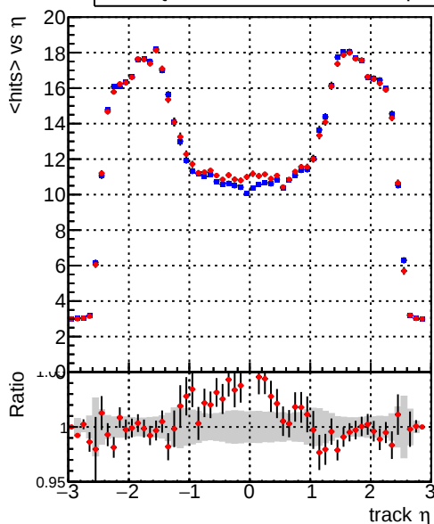
— DQM_CKF_TTbase — DQM_CKF_TT_retrainOldFiles125_v2_prelimWP2_epoch4 mean hits vs \eta
