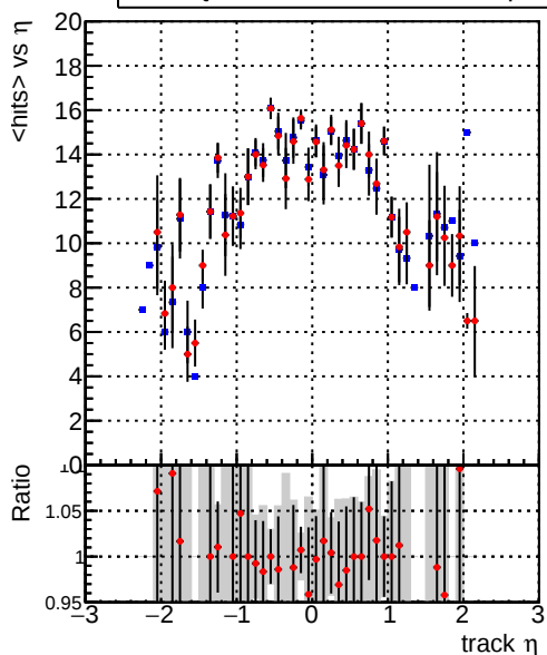
mean hits vs \eta Legend: DQM_CKF_TTbase (blue line with dots), DQM_CKF_TT_retrainOldFiles125_v2_prelimWP2_epoch4 (red line with dots)
