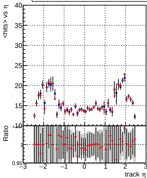
mean hits vs \eta — DQM_CKF_TTbase — DQM_CKF_TT_retrainOldFiles125_v2_prelimWP2_epoch4
