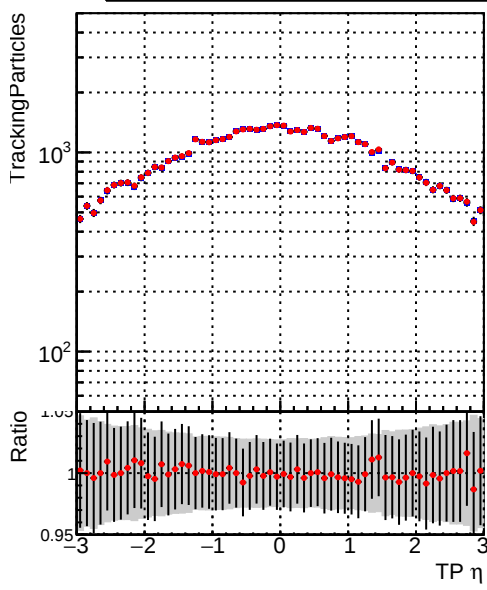
—•— DQM_CKF_TTbase —•— DQM_CKF_TT_retrainOldFiles125_v2_prelimWP2_epoch4
