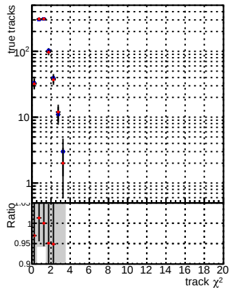
N of reco track vs. \chi^2 — DQM_CKF_TTbase — DQM_CKF_TT_retrainOldFiles125_v2_prelimWP2_epoch4
