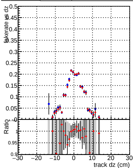
—●— DQM_CKF_TTbase —●— DQM_CKF_TT_retrainOldFiles125_v2_prelimWP2_epoch4
