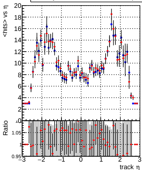
mean hits vs \eta Legend: DQM_CKF_TTbase (blue line with error bars), DQM_CKF_TT_retrainOldFiles125_v2_prelimWP2_epoch4 (red line with error bars)
