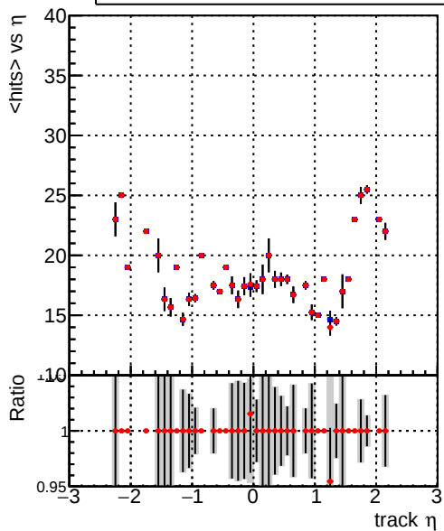
mean hits vs \eta Legend: DQM_CKF_TTbase (blue line with circles), DQM_CKF_TT_retrainOldFiles125_v2_prelimWP2_epoch4 (red line with circles)
