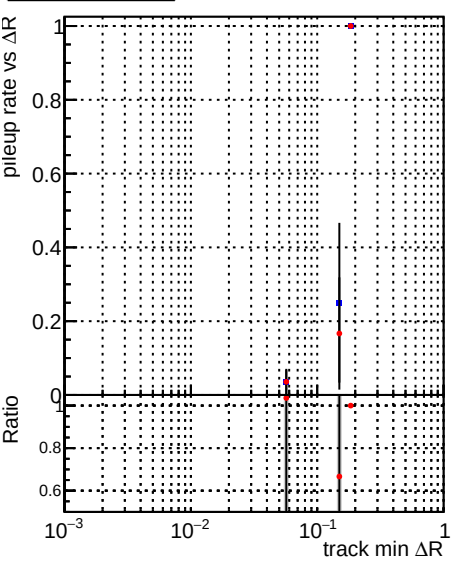
Legend: DQM_CKF_TTbase (blue dots), DQM_CKF_TT_retrainOldFiles125_v2_prelimWP2_epoch4 (red dots)
