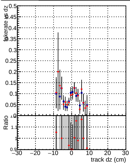
—●— DQM_CKF_TTbase —●— DQM_CKF_TT_retrainOldFiles125_v2_prelimWP2_epoch4
