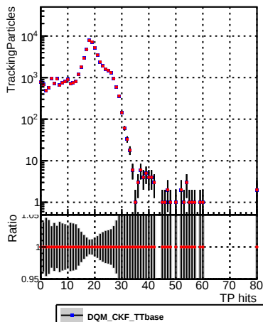
N of sim DQM_CKF_TTbase DQM_CKF_TT_retrainOldFiles125_v2_prelimWP2_epoch4
