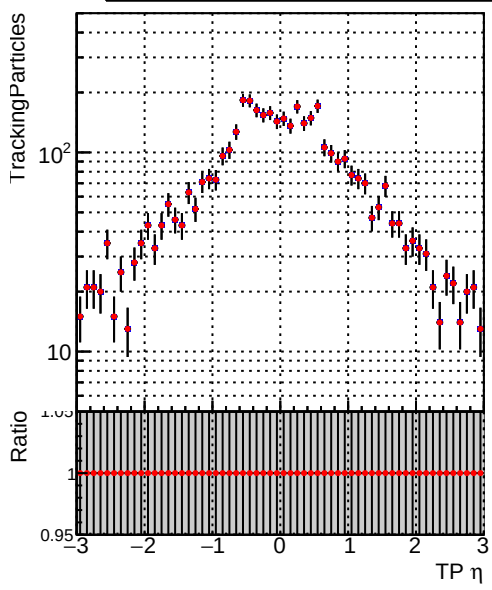
—●— DQM_CKF_TTbase —●— DQM_CKF_TT_retrainOldFiles125_v2_prelimWP2_epoch4
