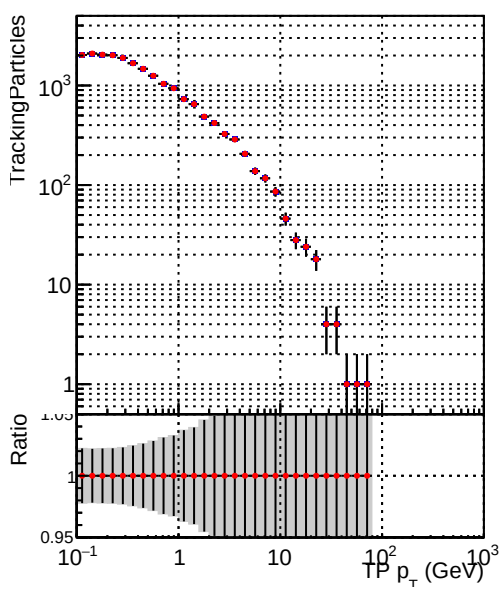
—●— DQM_CKF_TTbase —●— DQM_CKF_TT_retrainOldFiles125_v2_prelimWP2_epoch4
