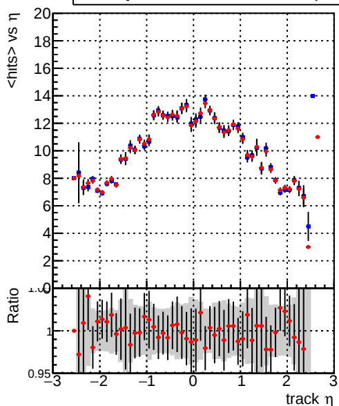
mean hits vs \eta Legend: DQM_CKF_TTbase (blue line), DQM_CKF_TT_retrainOldFiles125_v2_prelimWP2_epoch4 (red line)
