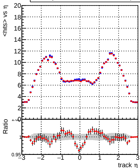
mean hits vs \eta Legend: DQM_CKF_TTbase (blue line), DQM_CKF_TT_retrainOldFiles125_v2_prelimWP2_epoch4 (red line with markers)
