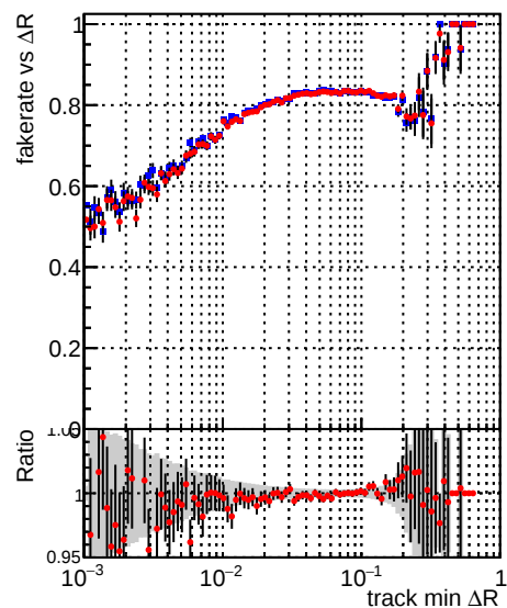
—•— DQM_CKF_TTbase —•— DQM_CKF_TT_retrainOldFiles125_v2_prelimWP2_epoch4
